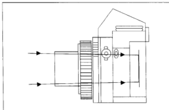
Fig. 9: Prime-Focus Photography.
