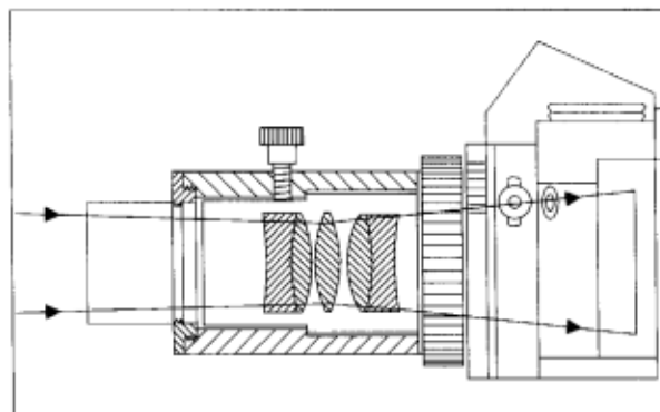
Fig. 10: Eyepiece-Projection Photography.
