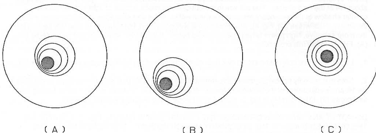
Fig. 5: Summary of the Collimation Procedure
