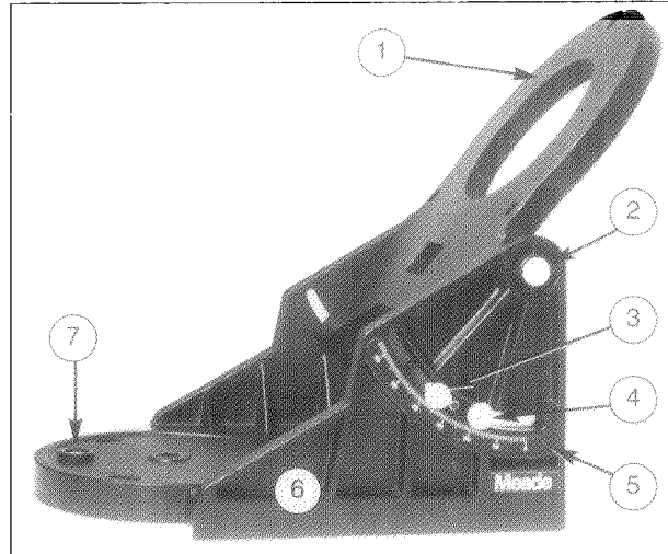
Fig. 7: Equatorial Wedge for 10" LX50 Telescope. (1) Tilt-Plate; (2) Attachment Screw; (3) Tilt Angle Locking Screw; (4) Fine Latitude Adjustment Mechanism; (5) Latitude Scale; (6) Wedge Body; (7) Bubble Level.
