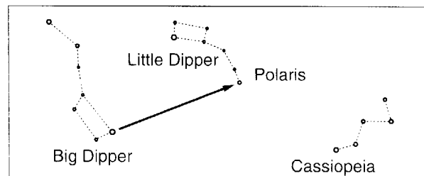
Fig. 17: Locating Polaris.
