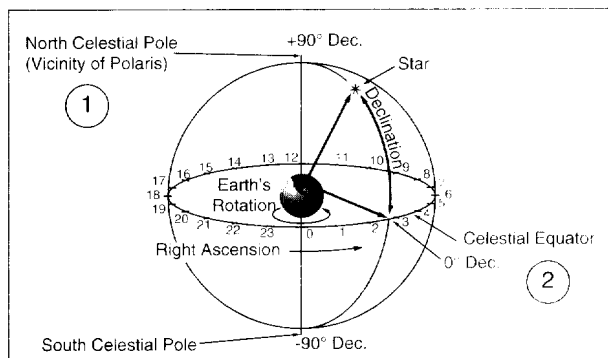
Fig. 16: Celestial Sphere.
